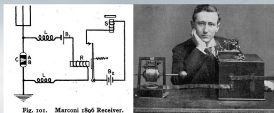
Fig. 101. Marconi 1896 Receiver.
